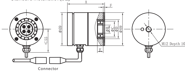
Standard installation (BZ)
