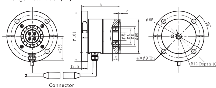
Flange installation (FL)
