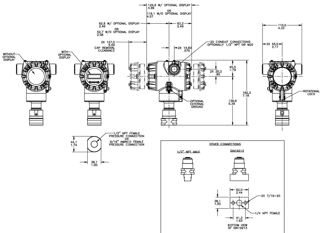
Figure 4– Typical mounting dimensions of STA72L & STA74L for reference
