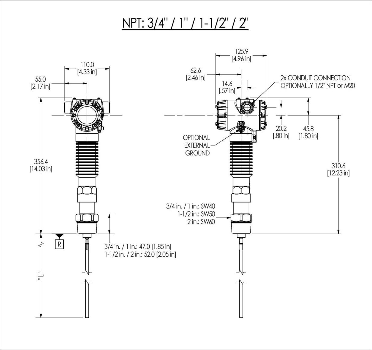
Figure 21 - SLG720 SmartLine Level with NPT fitting
