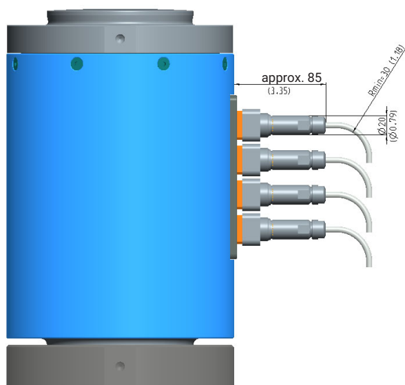
Version with bayonet connector
