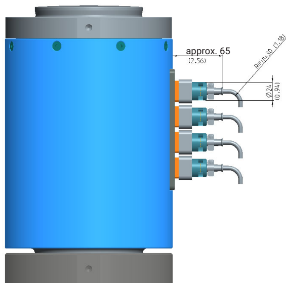
Version with threaded connector
