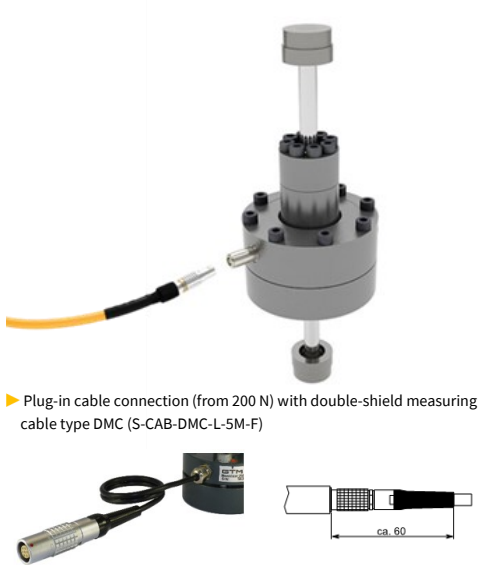
► Pluggable cable connection with external connection socket 5 N - 200 N
