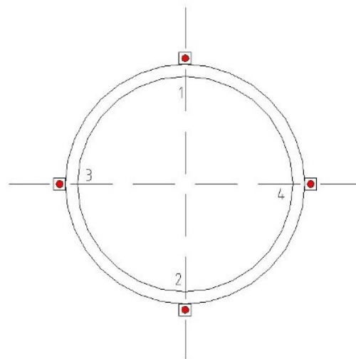
Figure 19: Four-gauge arrangement
