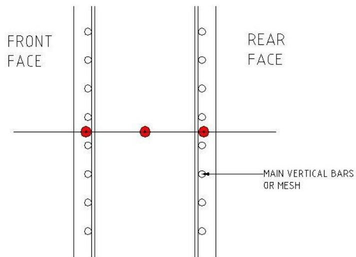
Figure 6: A horizontal section through a concrete wall in which strain gauges are positioned to measure bending of the wall.
