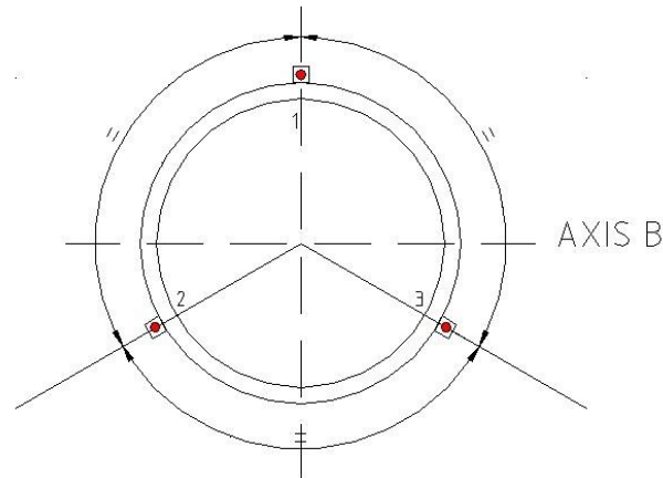
Figure 20: Three-gauge arrangement
